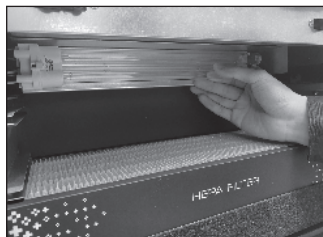
2 Replace the UV-C+ lamp
